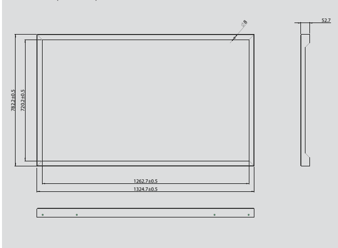
Dimensions (Unit: mm)
